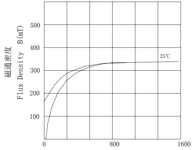
磁场强度 Magnetic Field Strength H (A/m)
